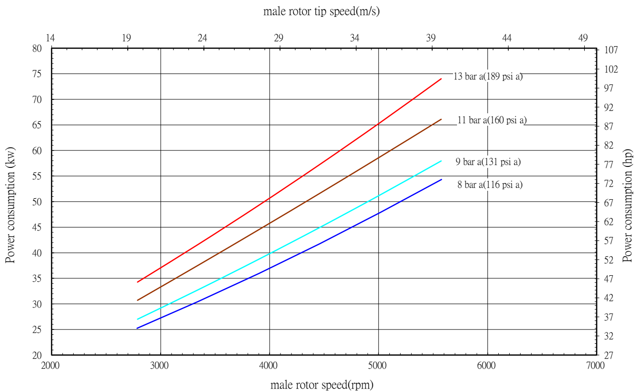
Oil injected screw compressor air end EU45(III)
