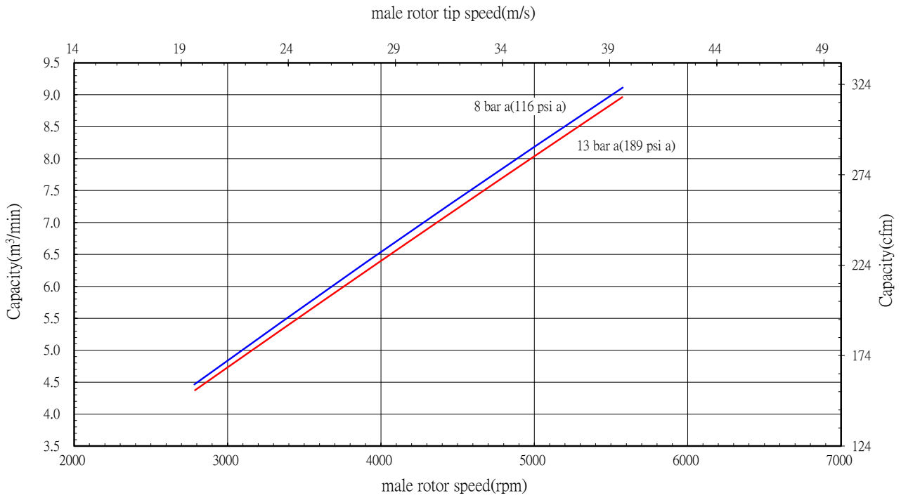
Oil injected screw compressor air end EU45(III)
